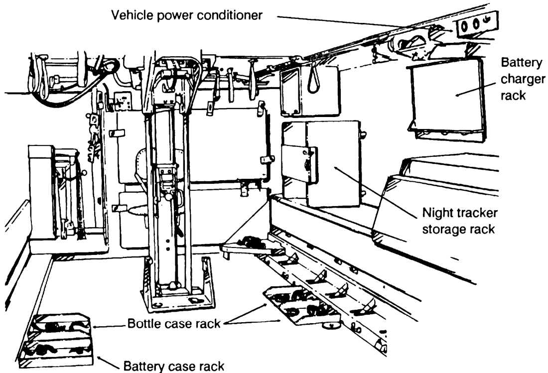
Figure 1-12. Vehicle storage kit.
