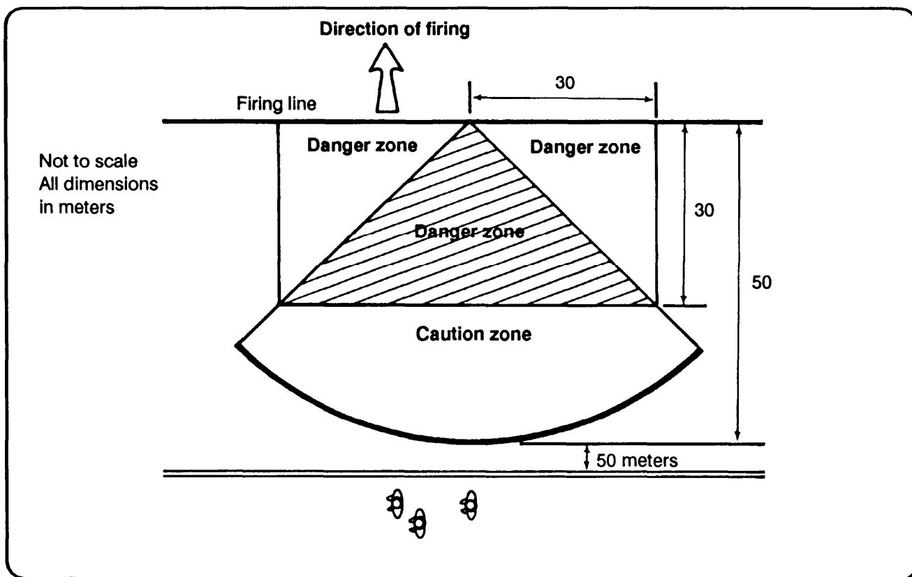
Figure 2-2. Personnel crossing 50 meters behind LES.
