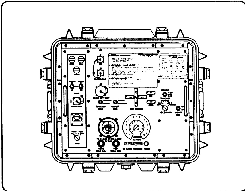
Figure 6-6. Monitoring set control panel.
