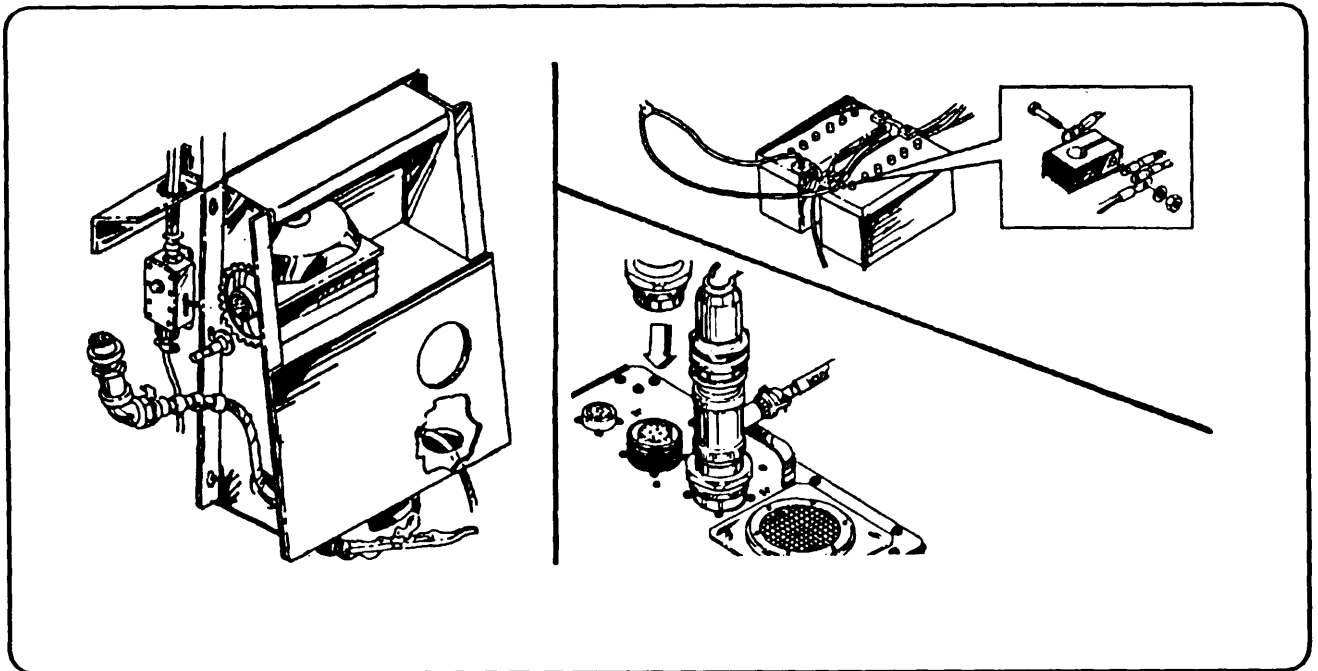
Figure 6-16. Ensuring cable routings are correct.
