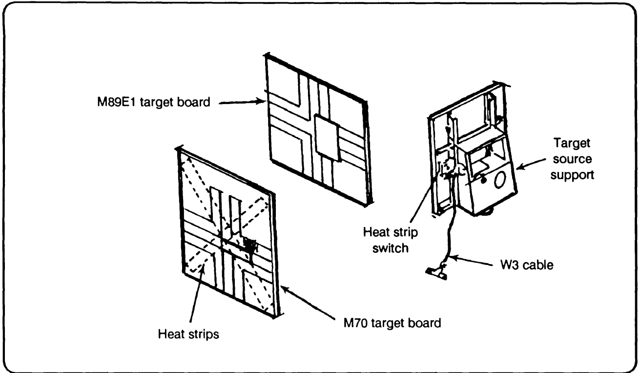
Figure 6-8. Infrared transmitting set.
