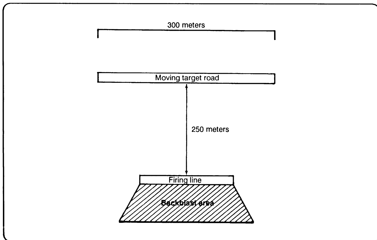
Figure 7-11. Target acquisition and tracking range.
