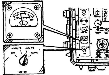
Figure 6-13. Conducting voltage test.
