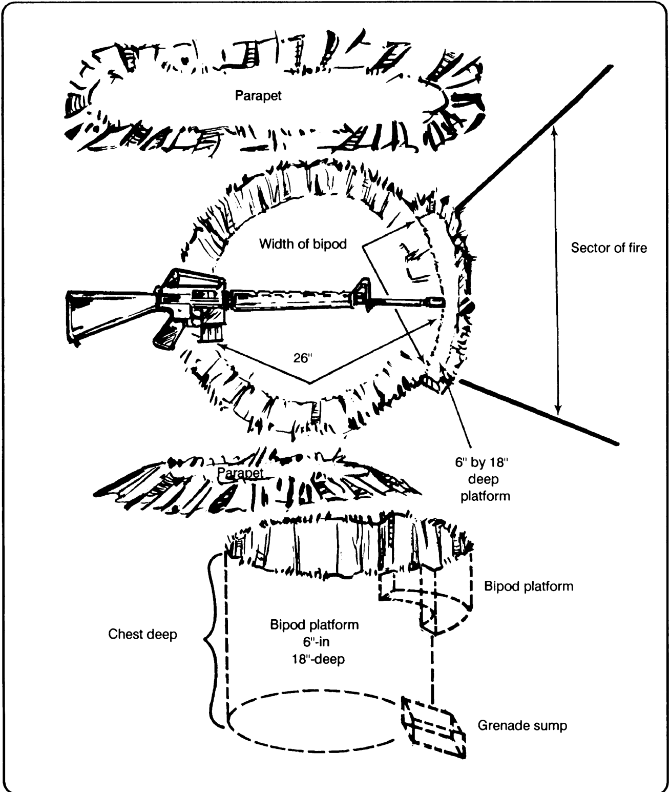
Figure 3-8. Construction of a one-man fighting position.
