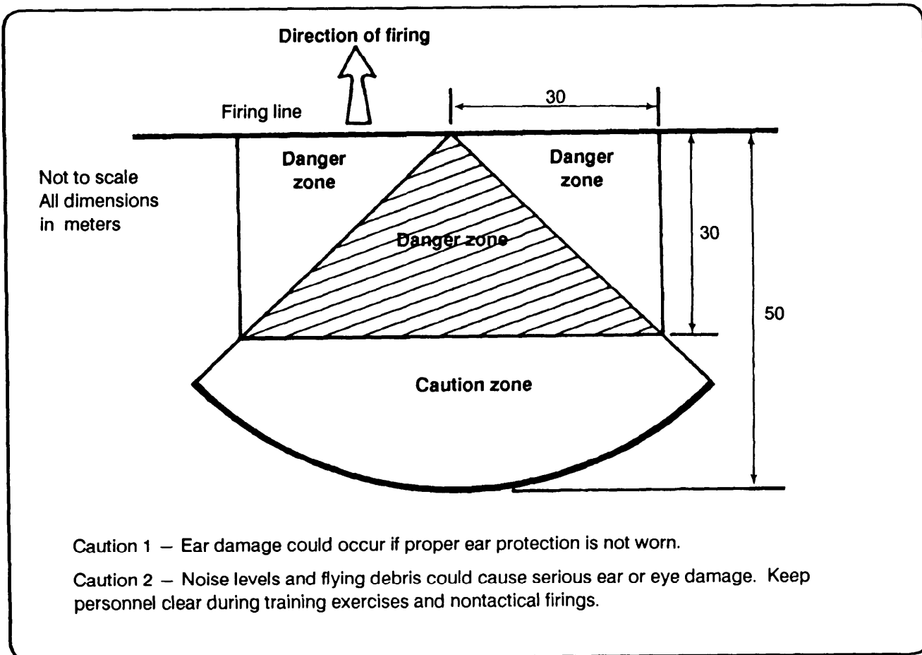
Figure 2-1. Dragon backblast area.
