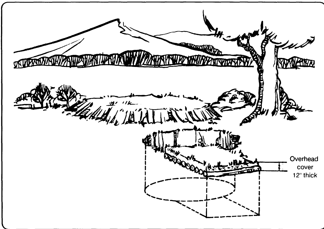
Figure 3-9. Construction of overhead cover.
