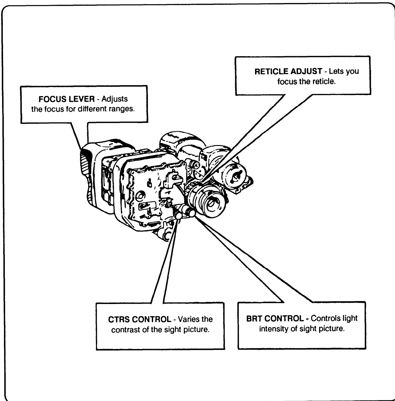
Figure 1-8. Night tracker controls.
