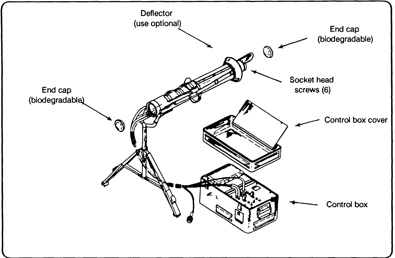
Figure 6-10. LES components.
