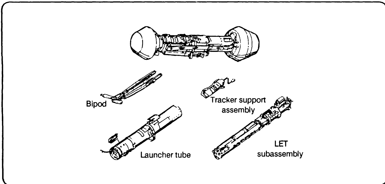
Figure 6-2. LET components.
