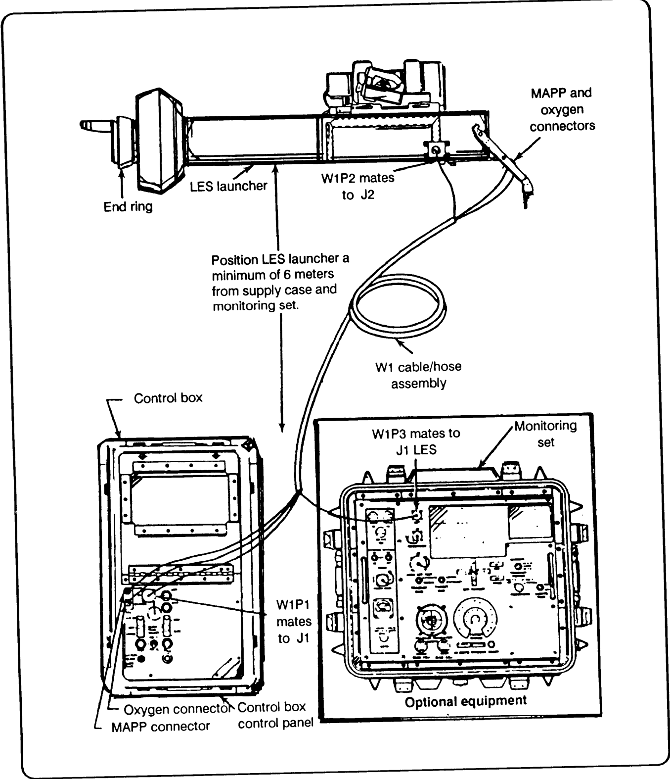
Figure 6-12. Mating the LES to the monitoring set.
