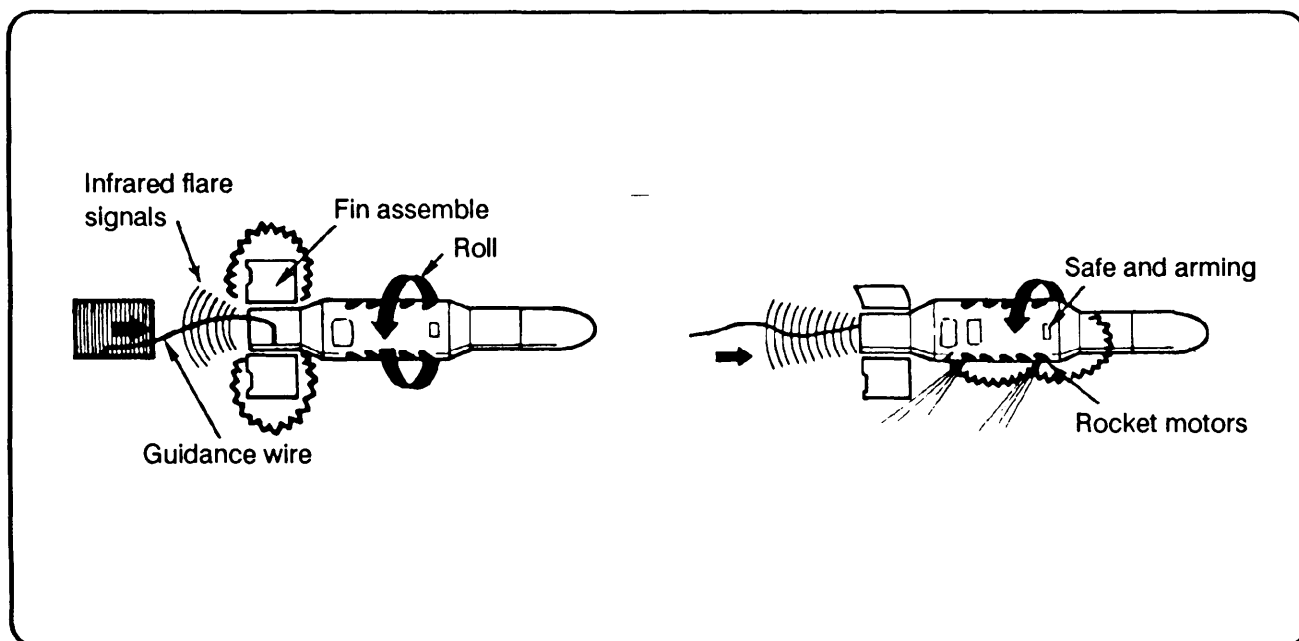
Figure 4-9. Dragon functioning concept.
